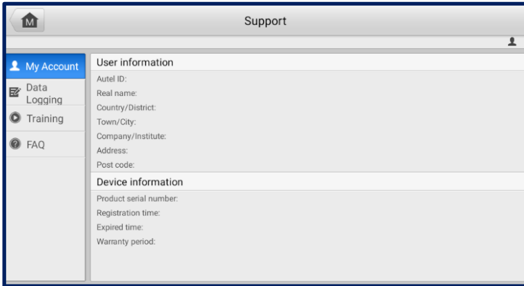
Figure 10-1 Support Screen
