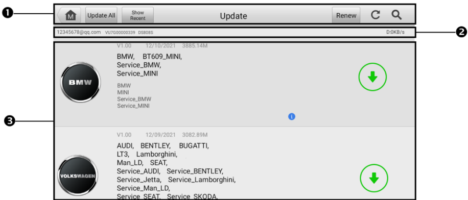
Figure 9-1 Update Screen
