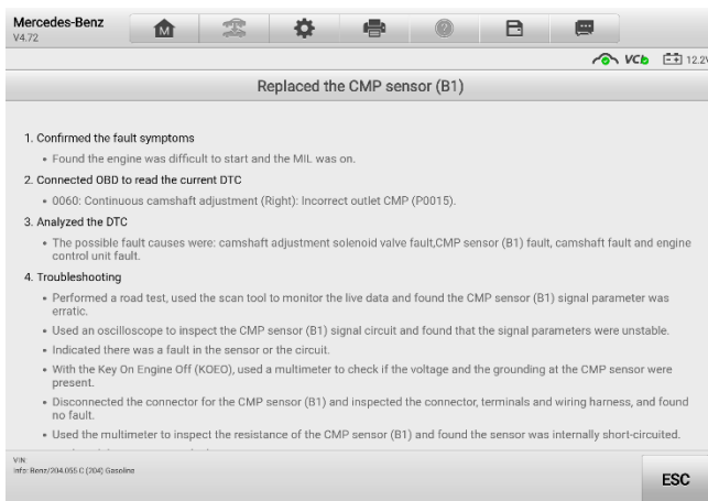
Figure 5-20 Repair Tips Description
