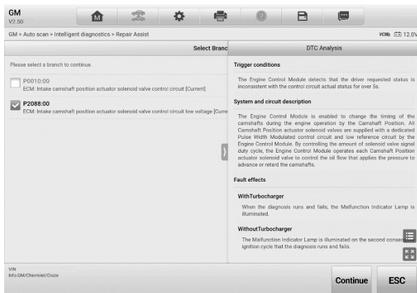
Figure 5-13 Repair Assist Screen 3
