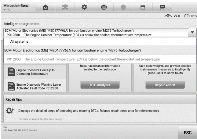
Figure 5-7 Vehicle System and Detected DTC(s) Screen
