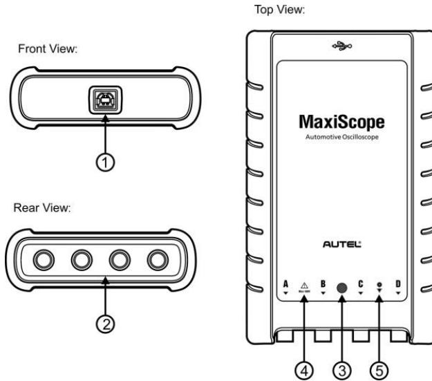
Figure 18-3 MaxiScope Front, Rear, and Top View
