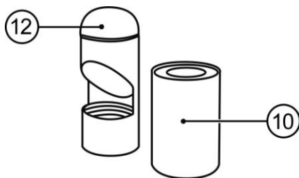
Fig. 3 5.5mm accessories
